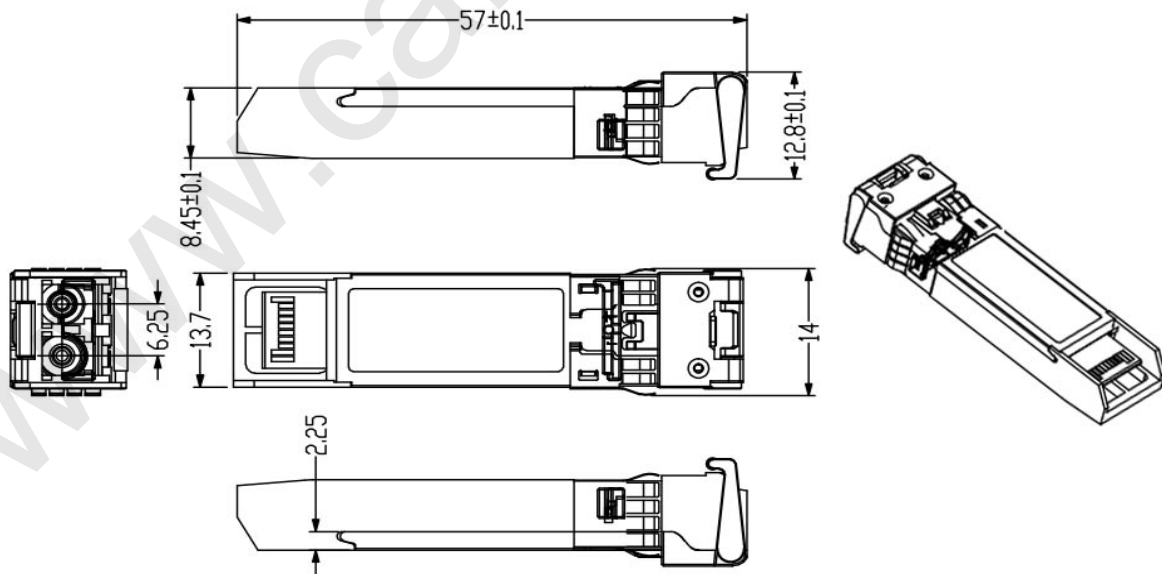
Mechanical Drawing
