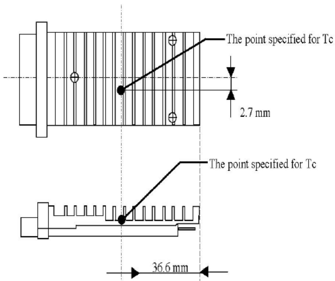
Figure 2 The Point Specified for Case Temperature ( T_c )
