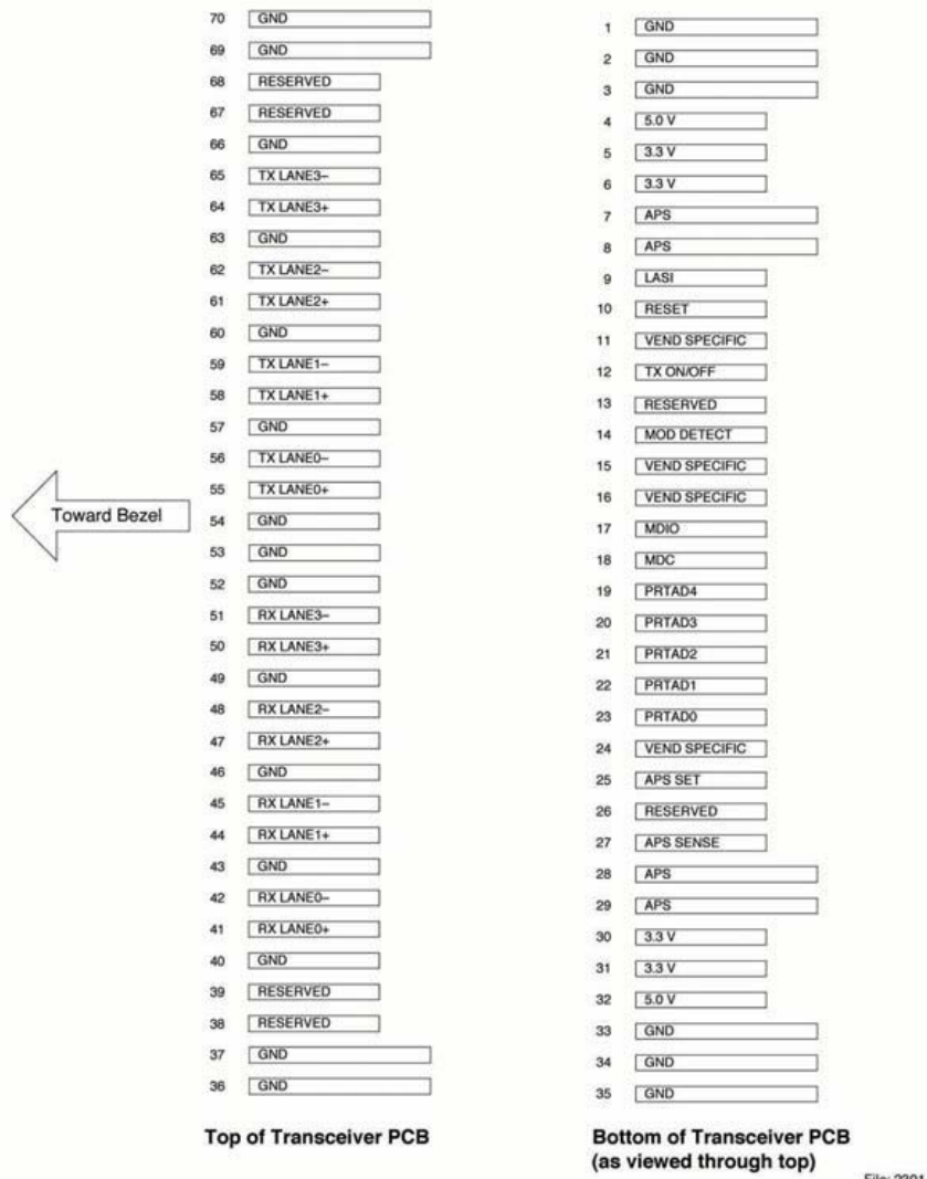
Fig 1-X2 Transponder Electrical Pad Layout
