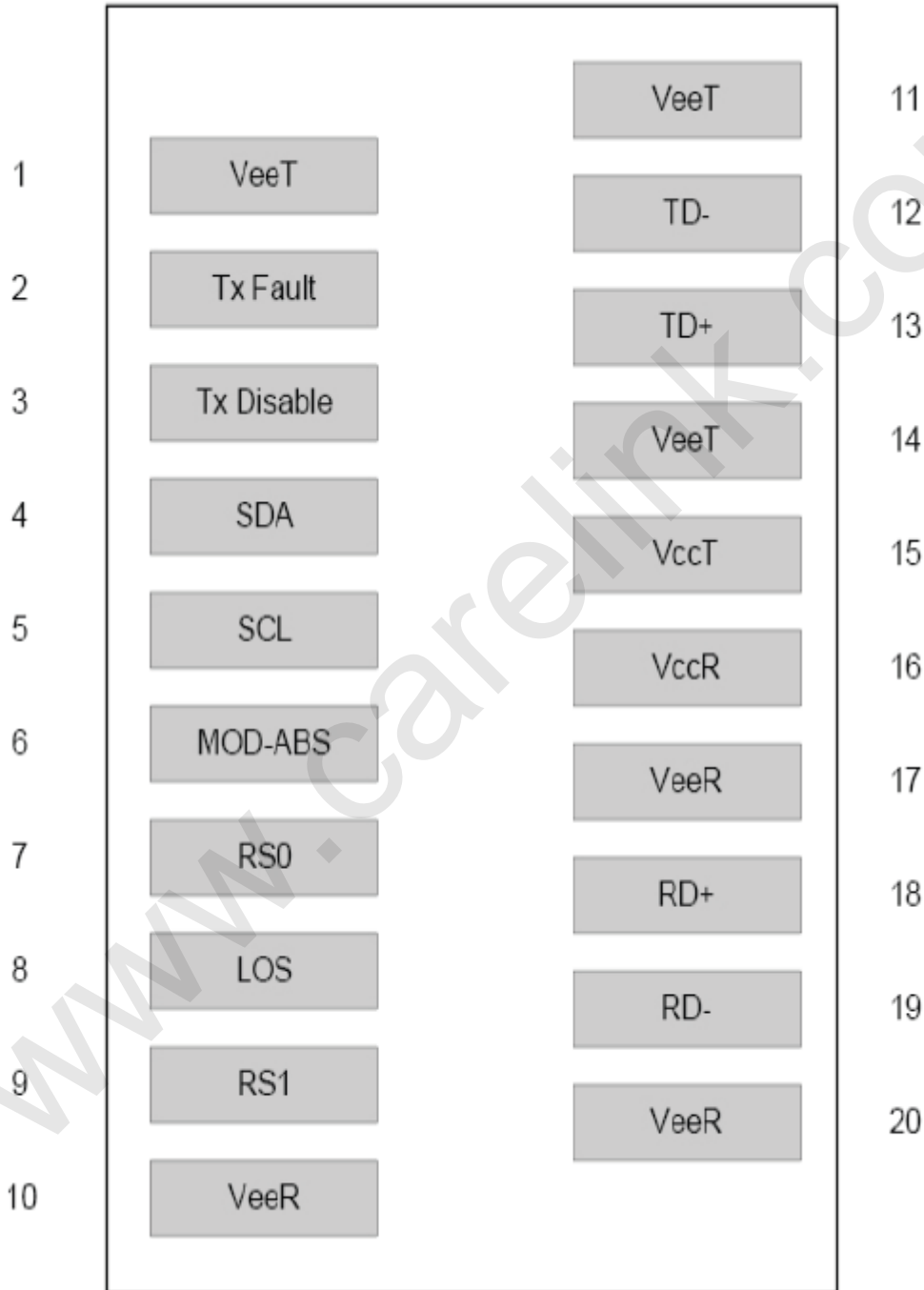
Diagram of Host Board Connector Block Pin Numbers and Name
