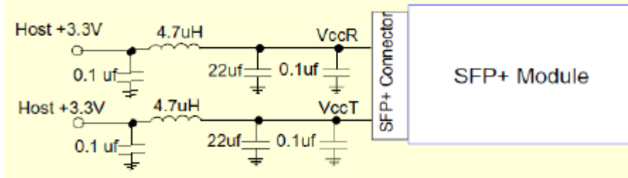
Recommended Host Board Power Supply Circuit
