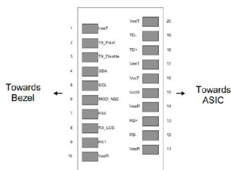
Pin-out of Connector Block on Host Board
